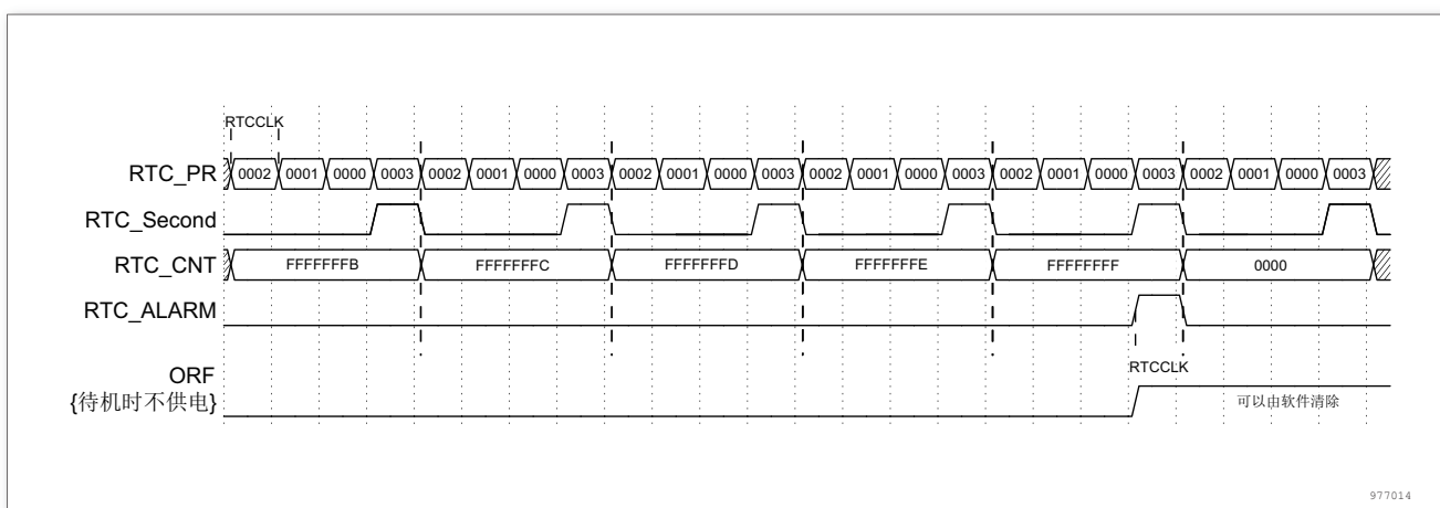
图 132. RTC 溢出波形图示例, PR = 0003
