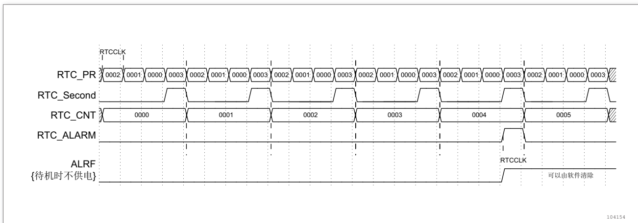
图 131. RTC 秒和闹钟波形图示例, PR = 0003, ALARM = 00004
