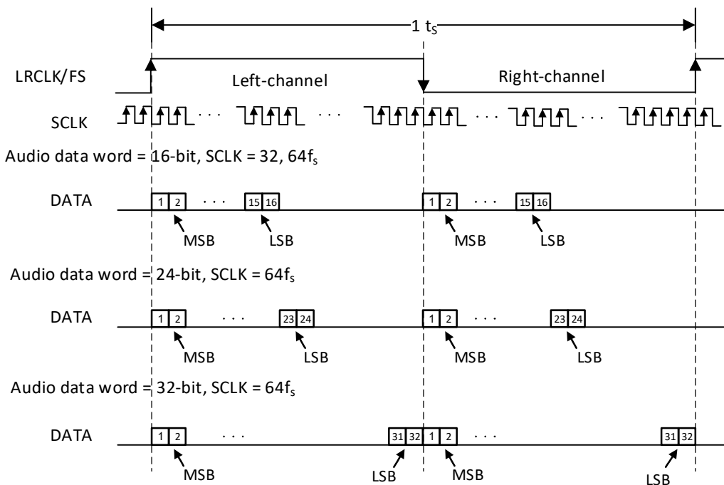
Figure 34 I 2 S Audio Data Format
