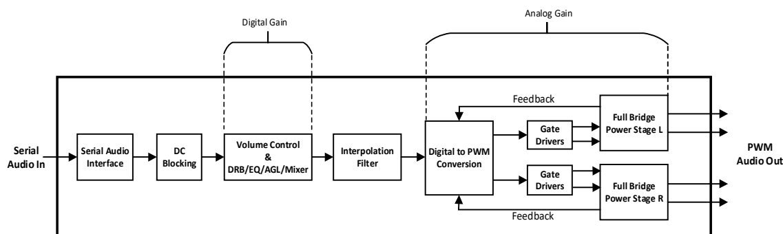
Figure 39 Gain Structure
