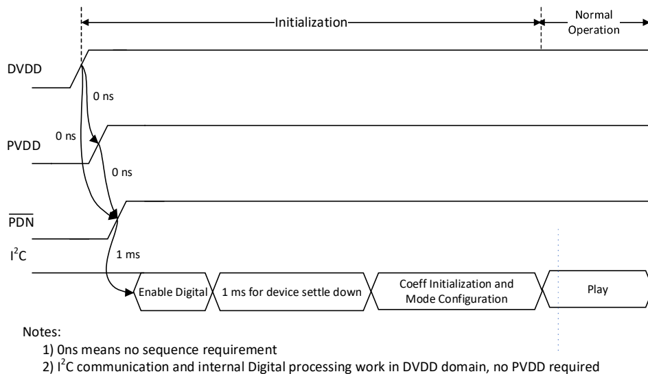
Figure 42 Start-up Sequence
